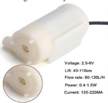
Fig. 3 Motor Pump
