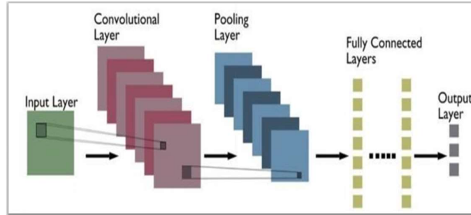
Fig.7 CNN Architecture
