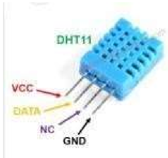
Fig. 2 Humidity Sensor
